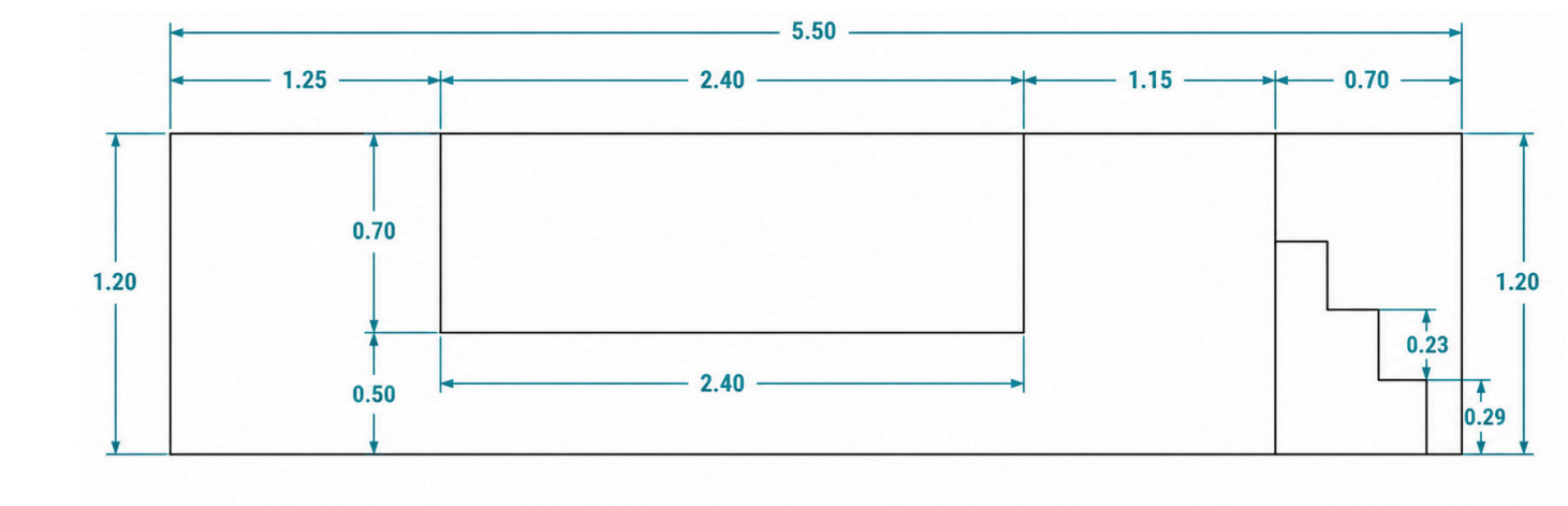
VISTA FRONTAL
